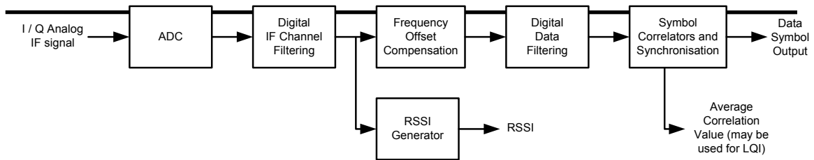
Figure 16. Demodulator Simplified Block Diagram
