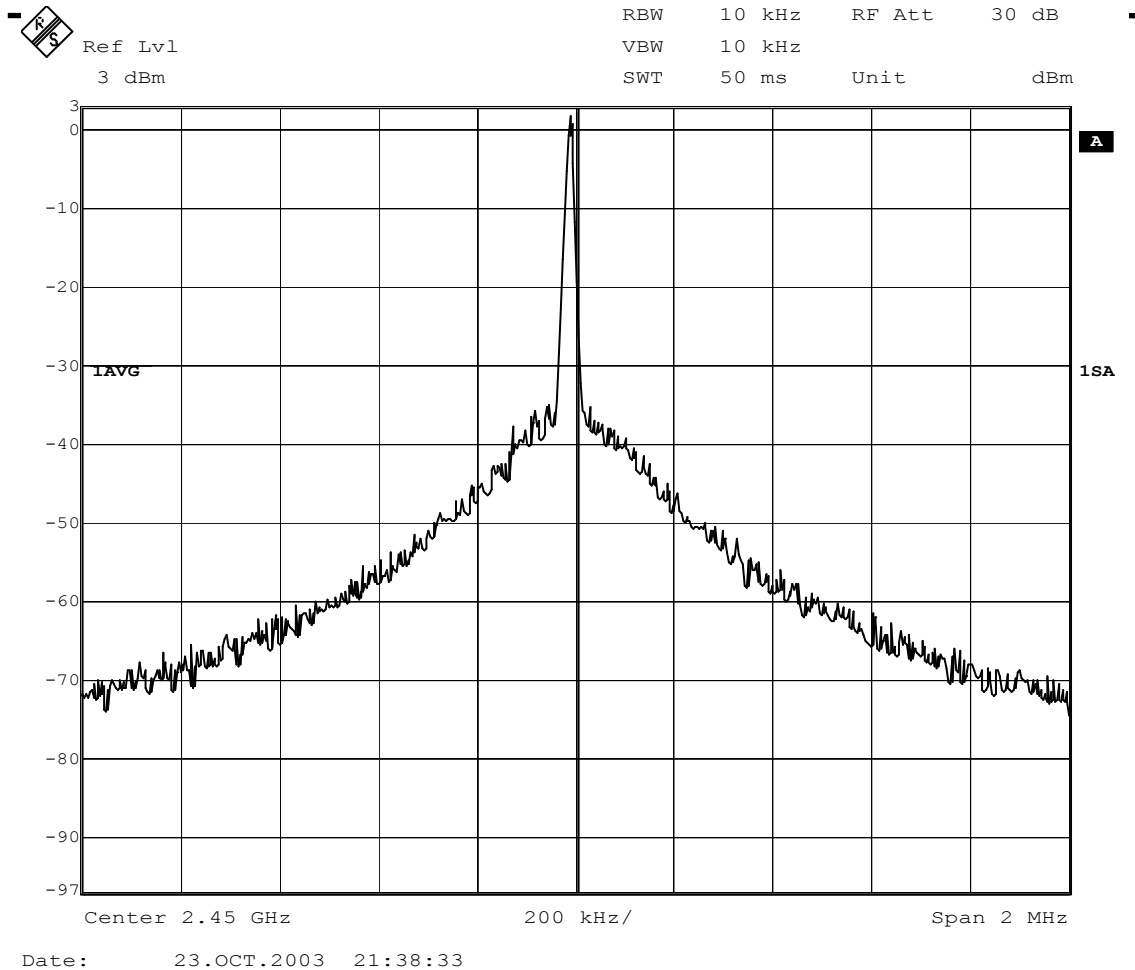
Figure 31. Single carrier output
