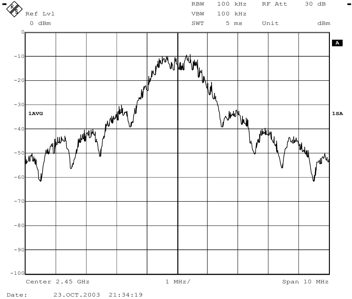
Figure 32. Modulated spectrum plot
