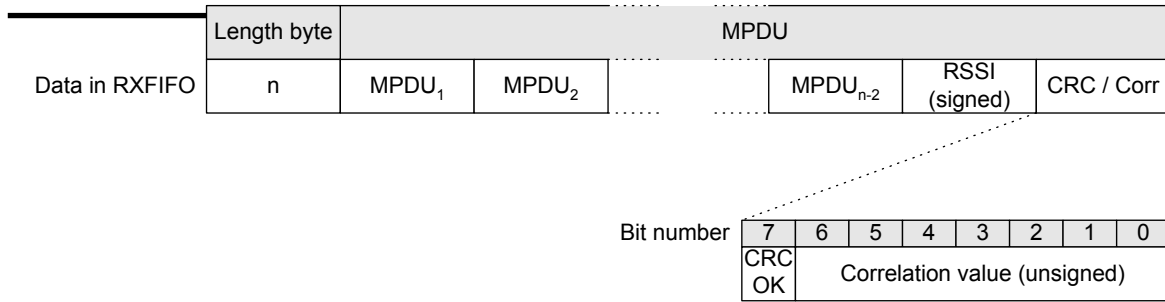
Figure 21. Data in RXFIFO when MDMCTRL0 . AUTOCRC is set
