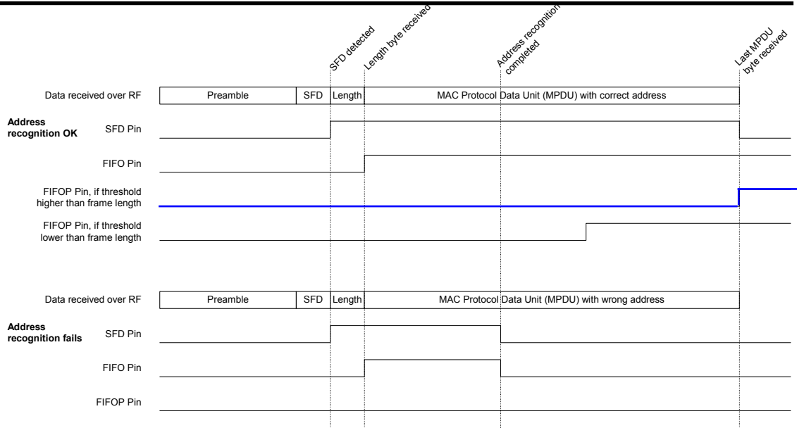
Figure 13. Pin activity examples during receive
